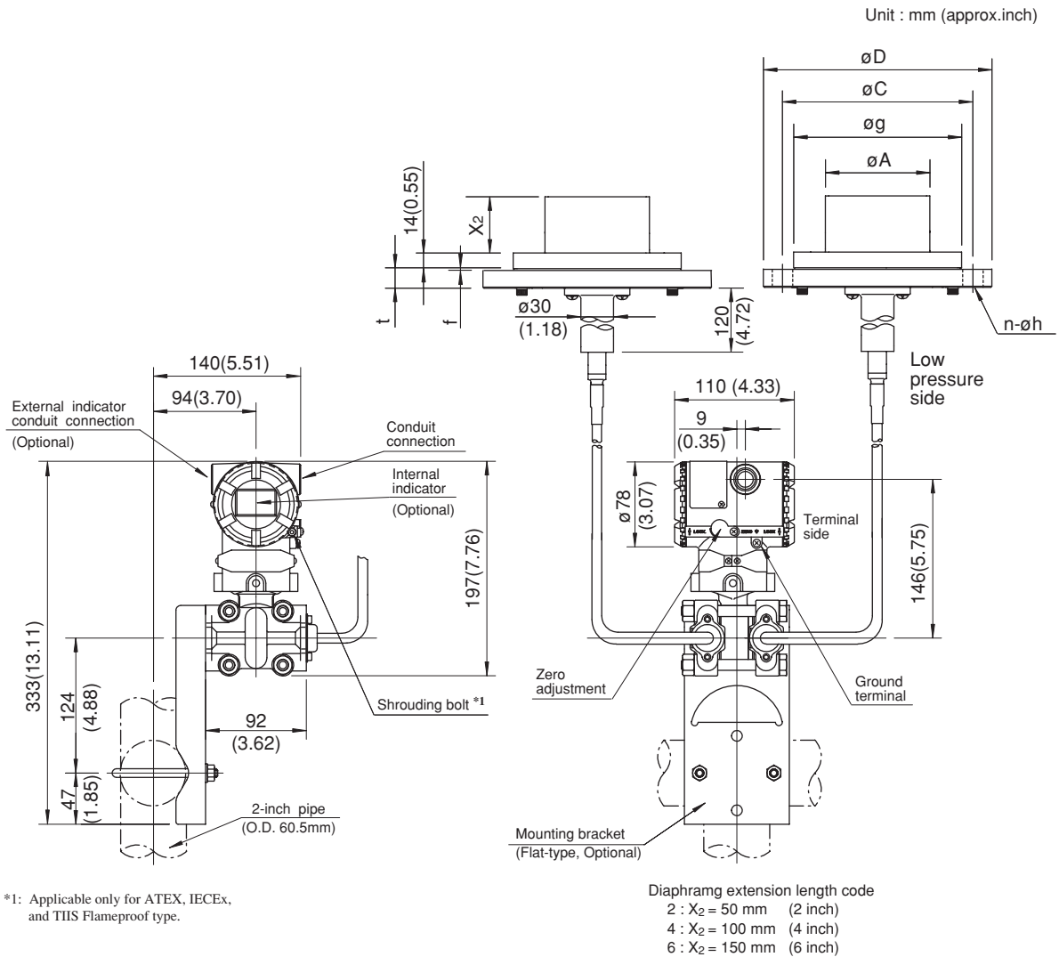
Process flange size : 4 inch (100 mm)
